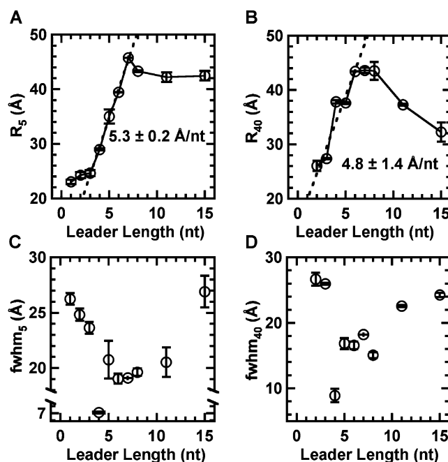
FIGURE 3: Time-resolved FRET experiments on the B. subtilis RNase P holoenzyme–pre-tRNA Asp complex. Upper panels: Mean donor–acceptor distance for the rhodamine-labeled K5C (A) and R40C (B) mutants as a function of 5' leader length (50 mM Tris-HCl–MES, pH 6.0, 20 mM CaCl 2 , 150 mM KCl, 10 mM imidazole, and 10 mM DTT at 25 °C). The dashed lines yield the indicated slopes for leaders between 3 and 7 nt and between 2 and 6 nt in length, respectively. Lower panels: Full width at half-maximum (fwhm) for the rhodamine-labeled K5C (C) and R40C (D) mutants as a function of 5' leader length. Error bars arise from two independent assays.
